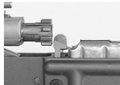
Rifle parts have been removed for illustration clarity. Check your rifle fully assembled.
